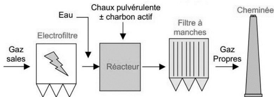
Figure II.3. Procédé semi-sec.
