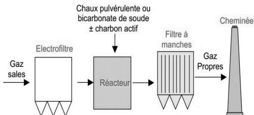
Figure II.4. Procédé sec.
